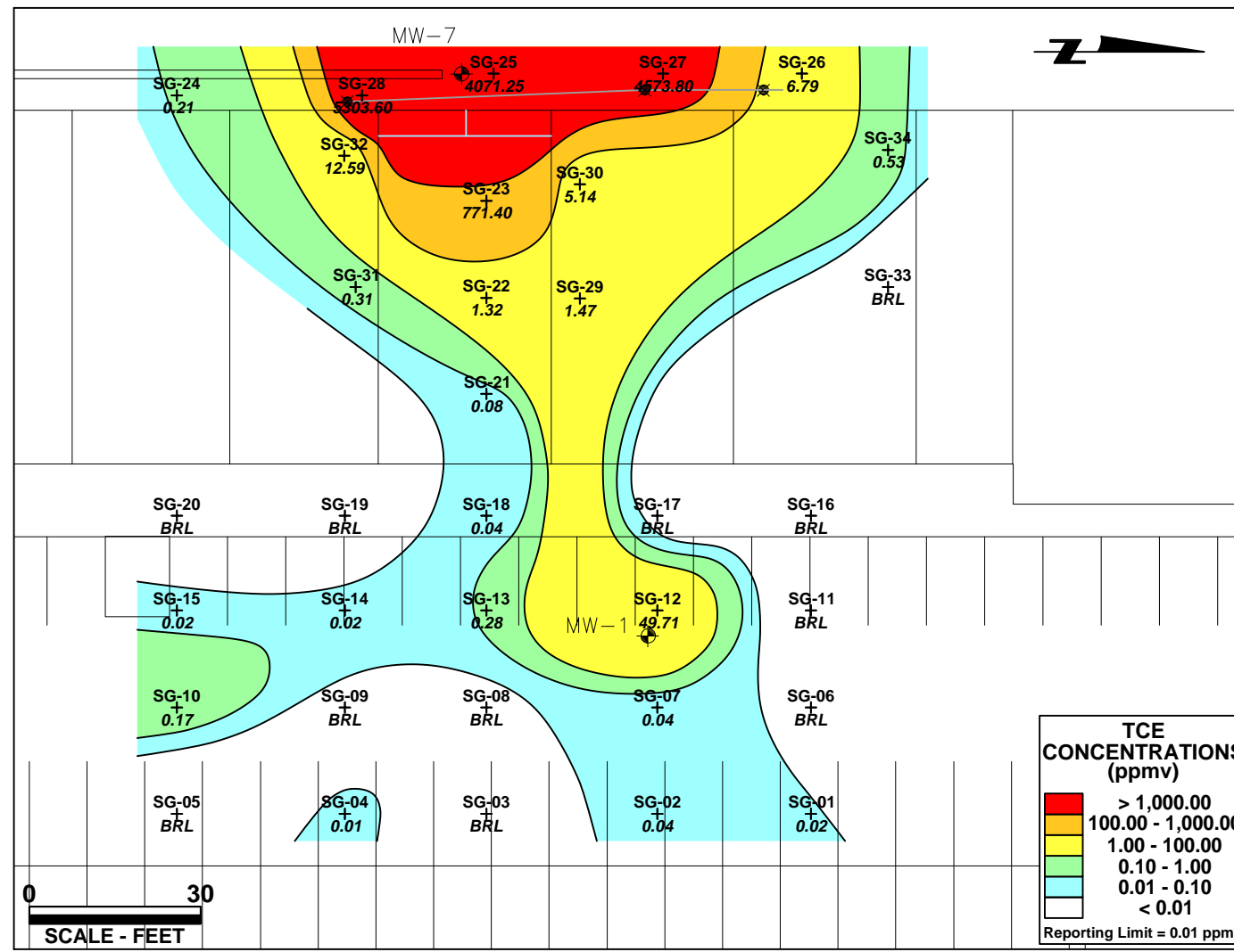
Trichloroethylene (TCE) Concentrations (ppmv)
