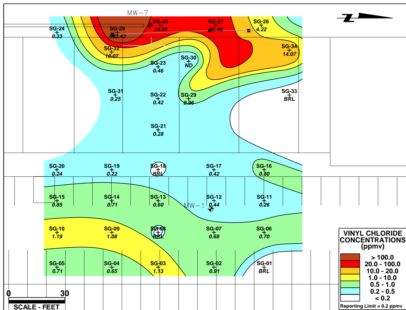
Vinyl Chloride (ppmv)
