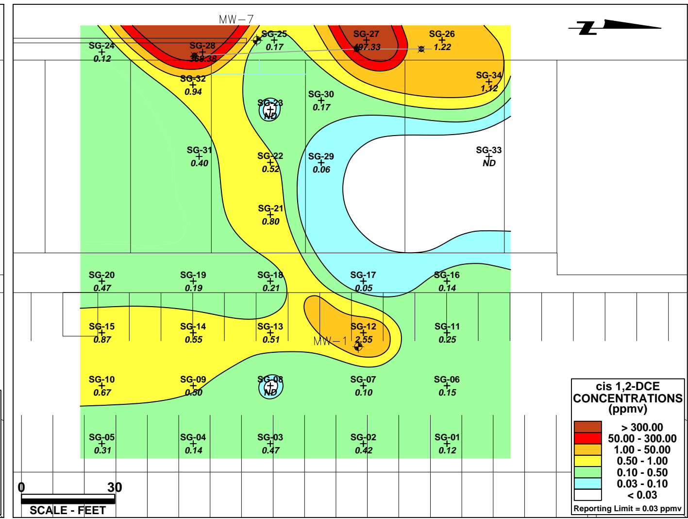
cis 1,2-DCE Concentrations (ppmv)
