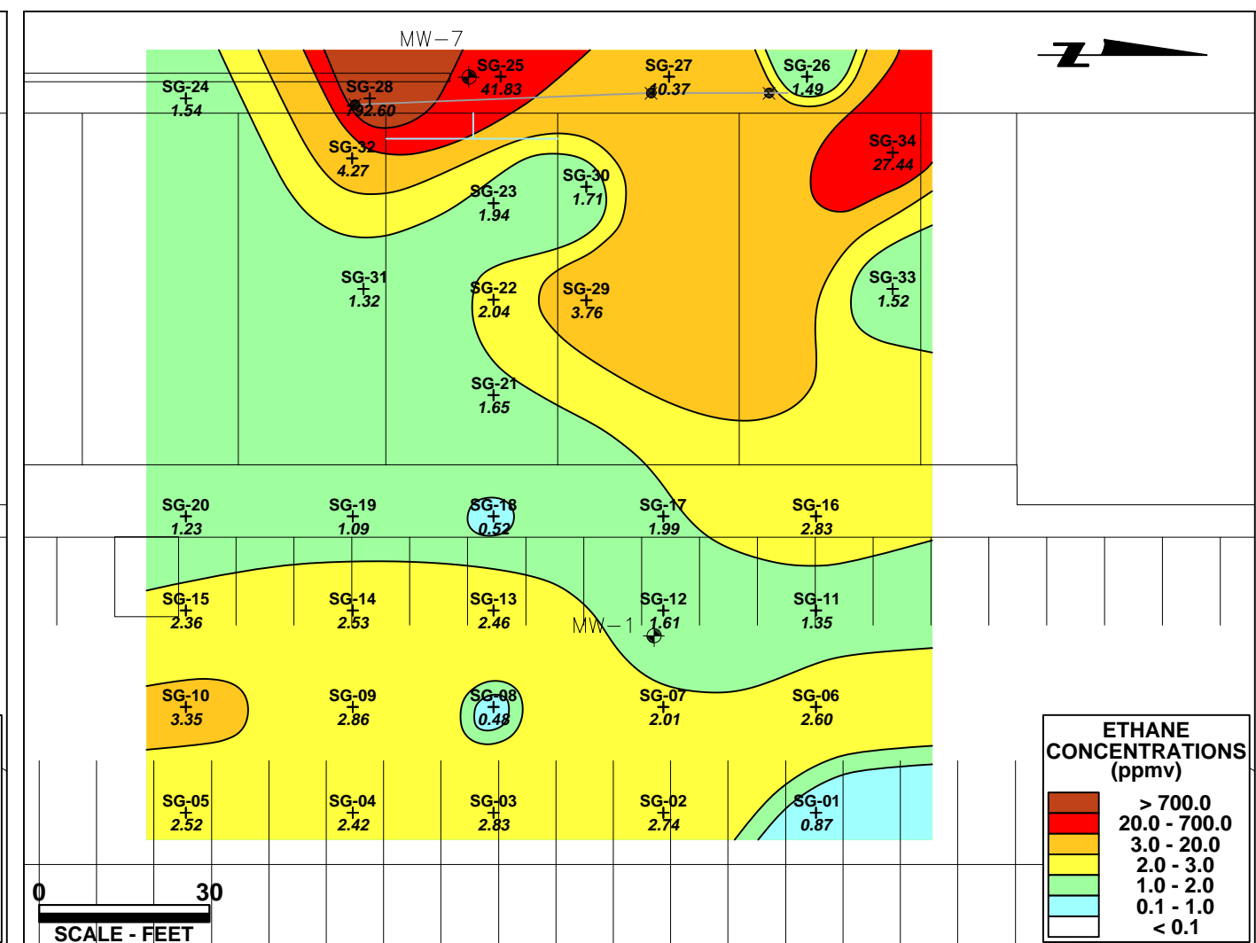
Ethane Concentrations (ppmv)
