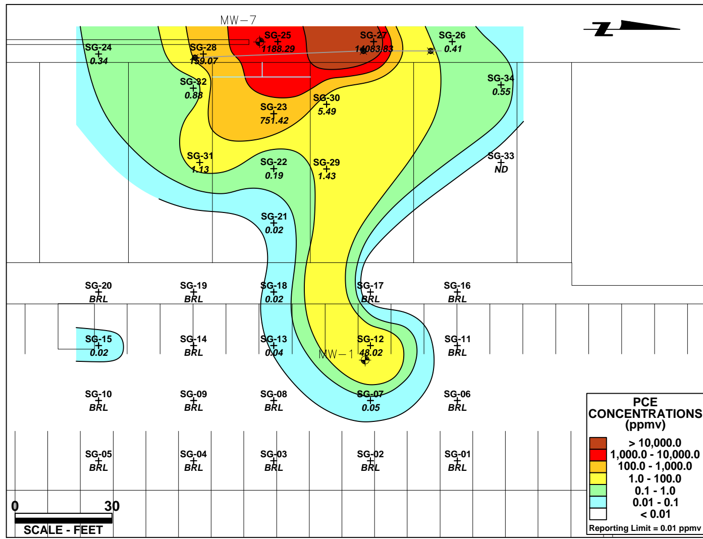
Tetrachloroethylene (PCE) Concentrations (ppmv)
