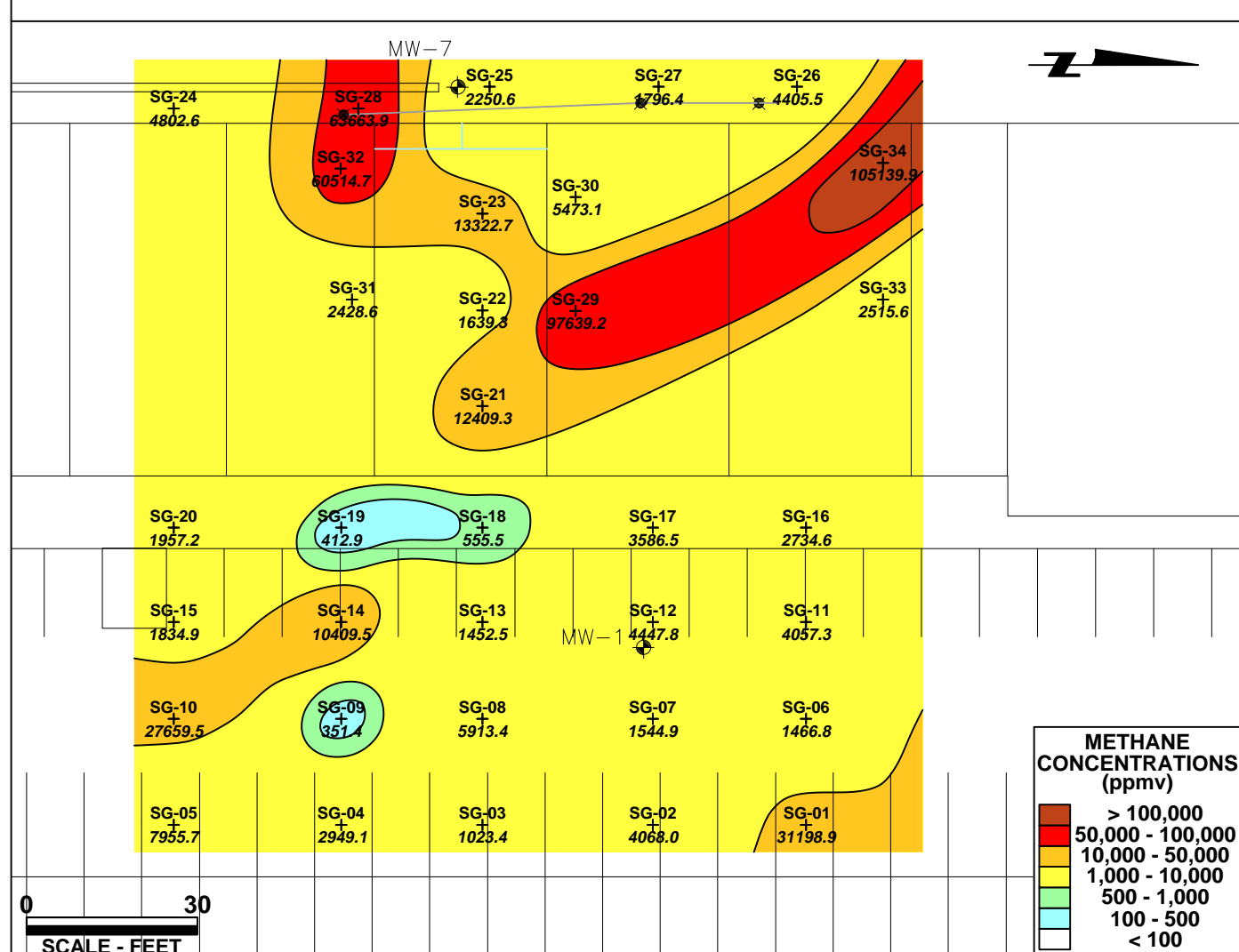
Methane Concentrations (ppmv)
