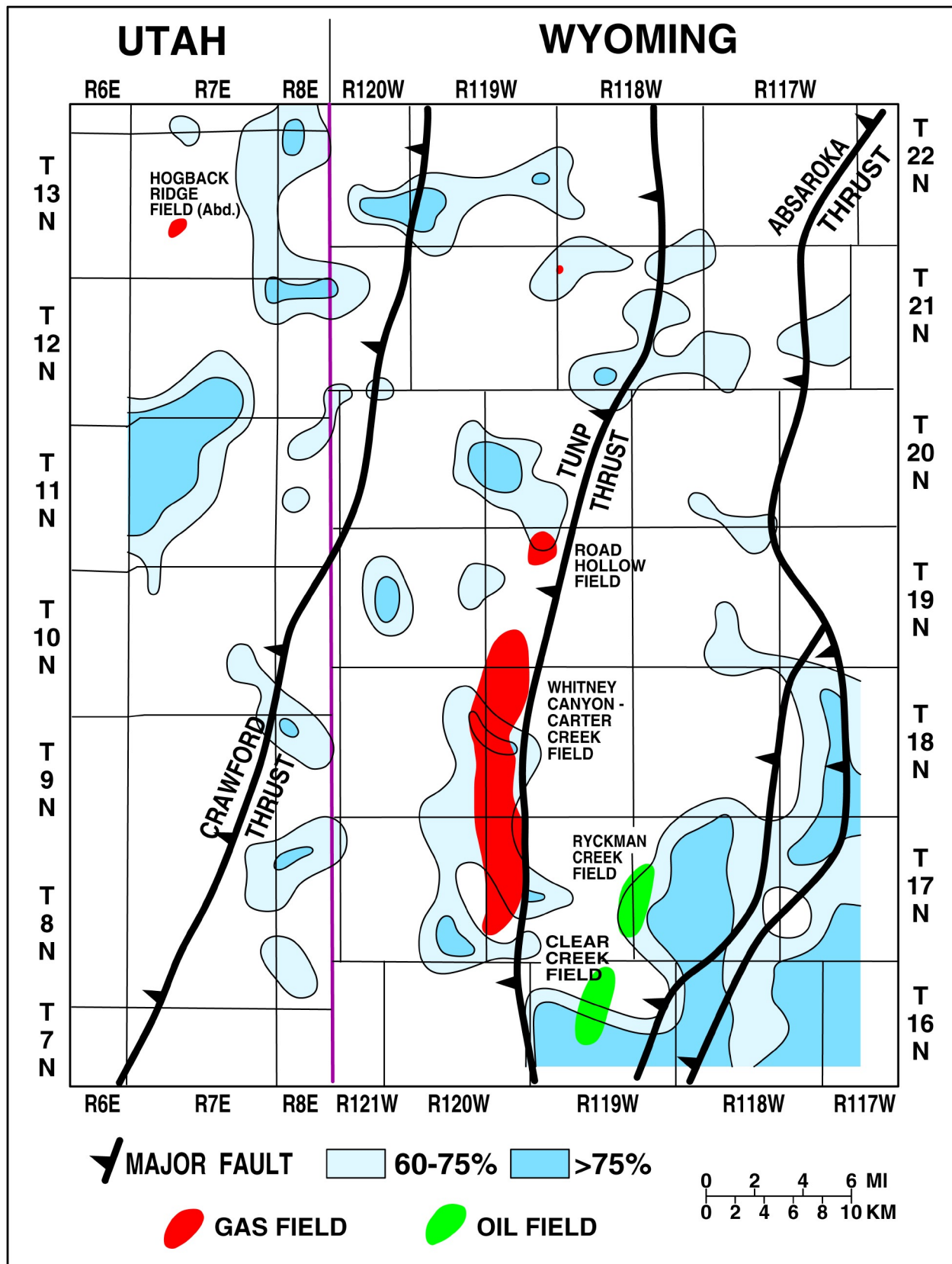
Fig. 5-44. Composite cell map in which the Monte Carlo simulations have been applied to methane, ethane, and propane anomalies, highlighting the regions where all three of these gases are above their respective medians.
