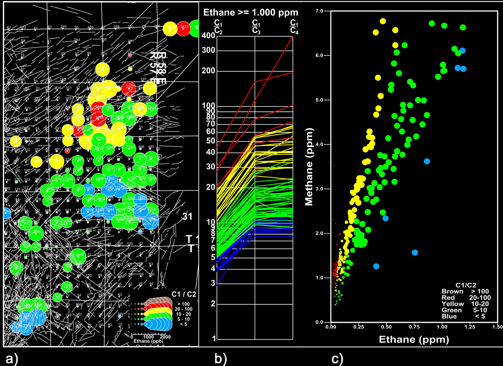
Fig. 5-40. a) Ethane compositional dot map for 1985 Currant Detail, Railroad Valley, Nevada; b) Pixler-type diagram characterisation of anomalous soil gas hydrocarbons associated with known oil fields in Railroad Valley, Nevada; c) Methane/Ethane Scatter Plot for 1985 Currant Detail Soil Gas Data, Railroad Valley, Nye County, Nevada
