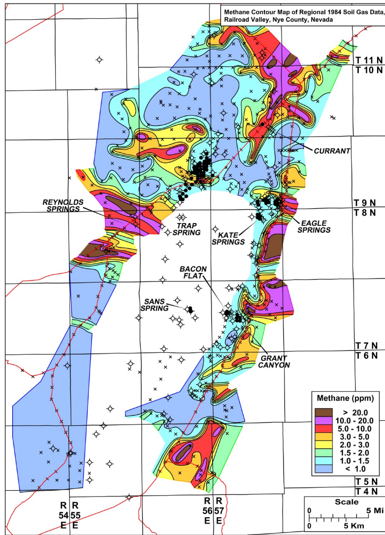
Fig. 5-35. a) Methane Contour Map of Regional 1984 Soil Gas Data, Railroad Valley, Nye County, Nevada; b) Propane Contour Map of Regional 1984 Soil Gas Data, Railroad Valley, Nye County, Nevada.
