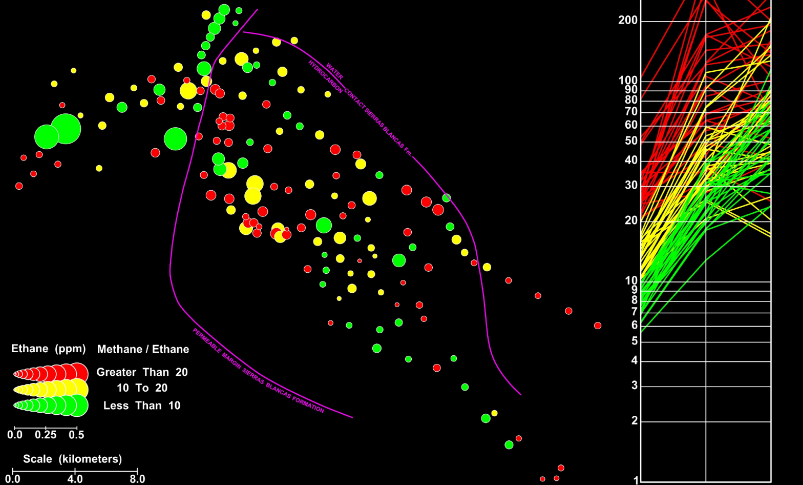
Fig. 5-32. Spatial distribution of soil gas hydrocarbons at Loma de La Lata oil and gas field, Argentina; dot size indicates ethane concentration; dot color indicates C1/C2 ratio, green (oil), yellow (intermediate), and red (gas).
