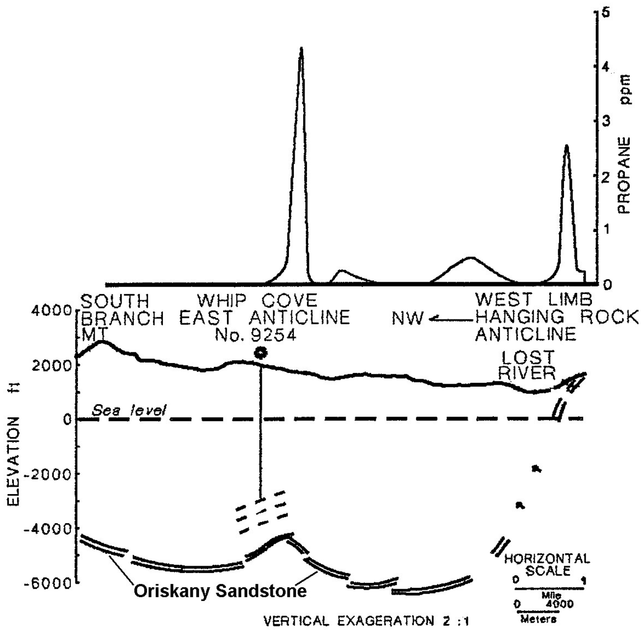
Fig. 5-30. Cross-section through the Lost River oil field, West Virginia, and profile of propane in soil gas (reproduced with permission from Matthews et al., 1984).
