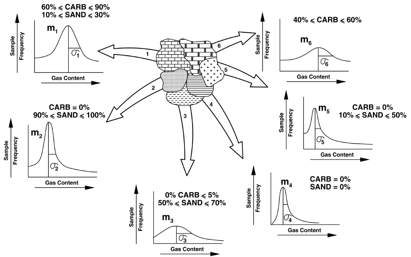
Fig. 5-26. Scheme for lithological classification of samples prior to interpretation of gases released by acid extraction (reproduced with permission from Poll, 1975).
