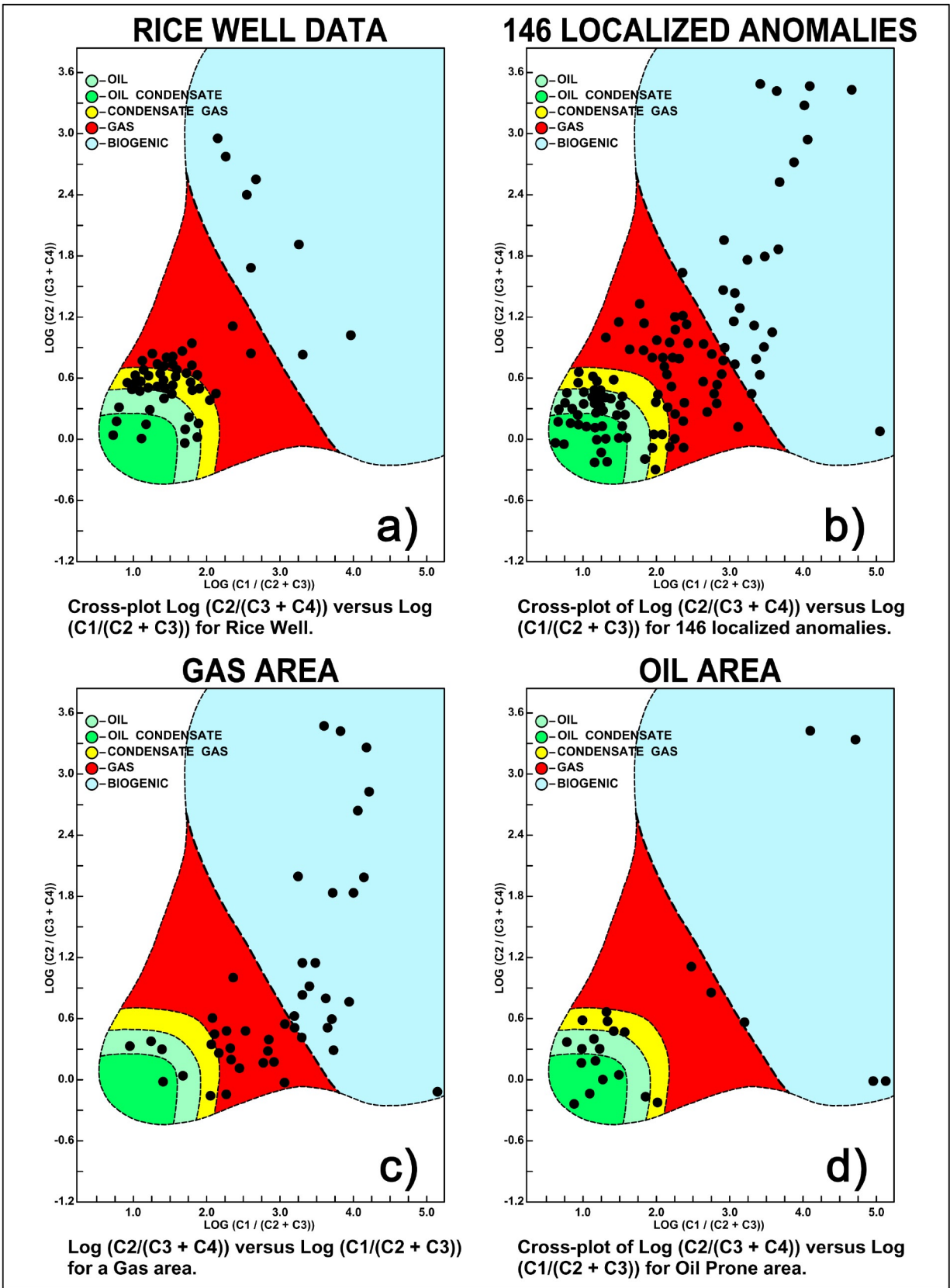
Fig. 5-24. Crossplots of the compositions of dissolved gases anomalies from offshore Louisiana reservoirs and sniffer surveys: a) Rice well gases; b) Typical marine sniffer gases anomalies; c) marine sniffer gases from a gas area; d) marine sniffer gases from an oil area.
