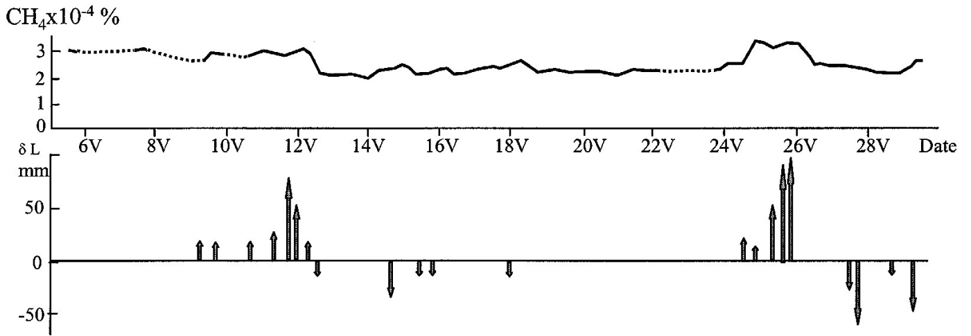
Fig. 5-16. Variations in methane concentration in air with crustal displacement in a seismically-active region (reproduced with permission from Antropov et al., 1981).
