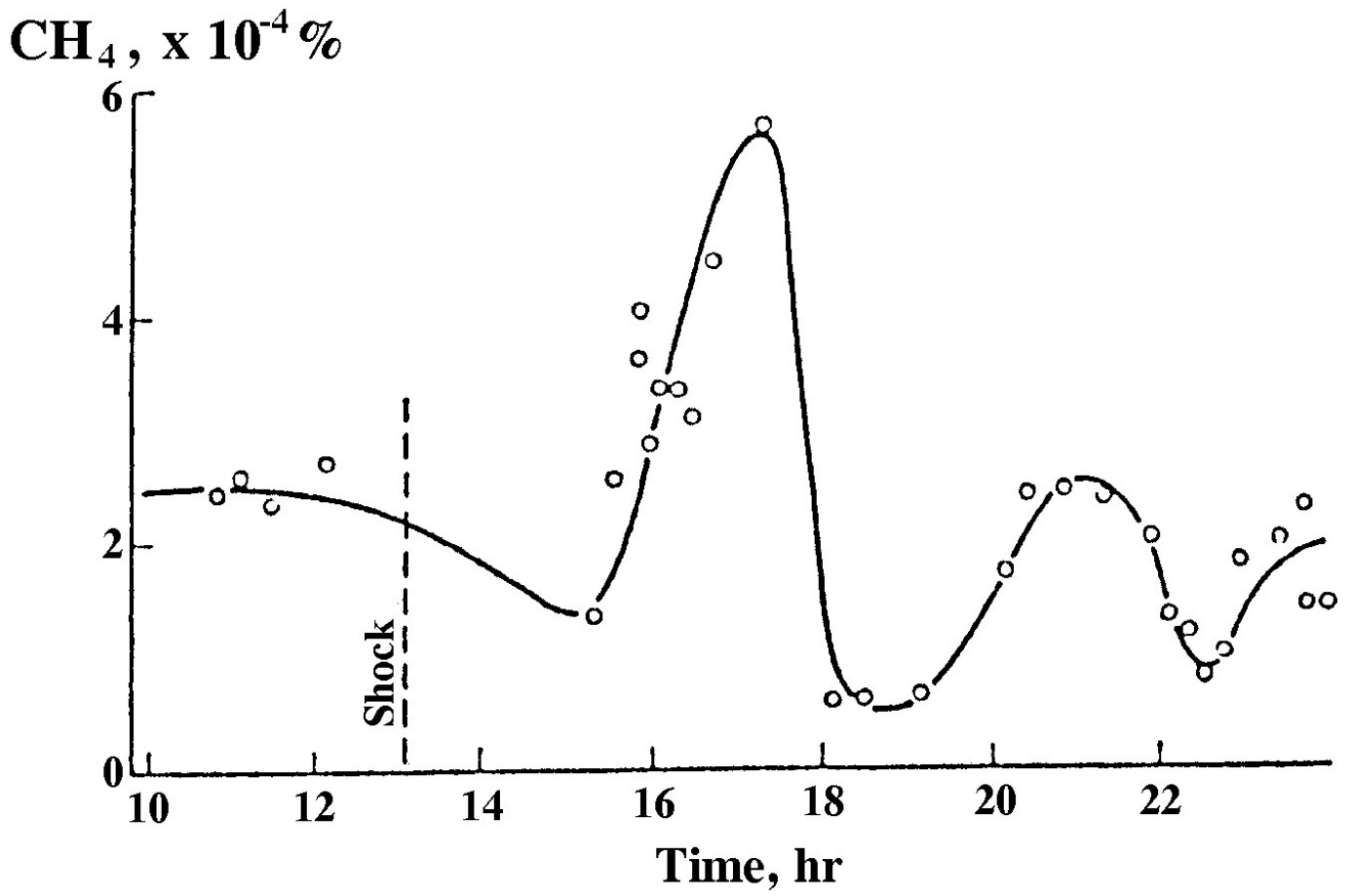
Fig. 5-15. Variations in methane concentration in air as a result of seismic shock to the ground (reproduced with permission from Antropov, 1981).
