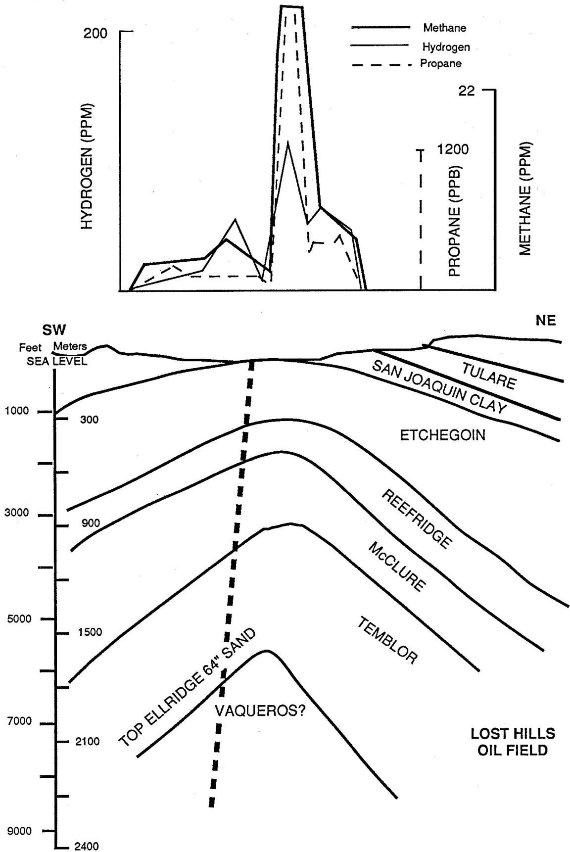
Fig. 5-13. Relation of near-surface gases to proposed deep fault adjacent to Lost Hills oil field, San Joaquin Basin, California (reproduced with permission from Jones and Drozd, 1983).
