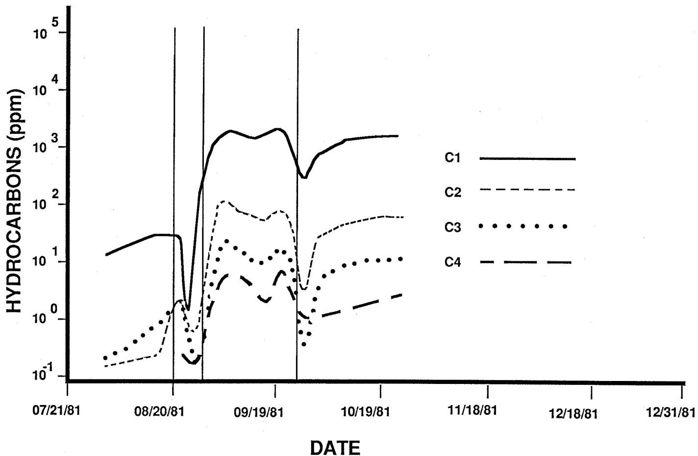
Fig. 5-9. Arrival at a surface well of hydrocarbon gases following a subsurface coal-burn experiment at Rawlins, Wyoming (reproduced with permission from Jones and Thune, 1982).
