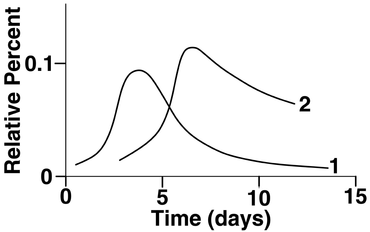
Fig. 5-8. Differentiation of methane (1) and heavy hydrocarbons (2) during migration from an artificial source (reproduced with permission from Sokolov, 1971 b).
